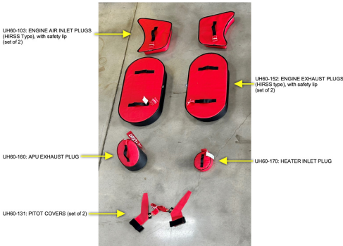
Sikorsky UH-60A Plug Set
