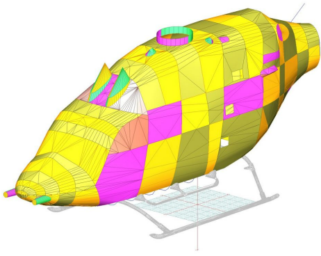
Bell 429 Main Body Cover, 3D model
