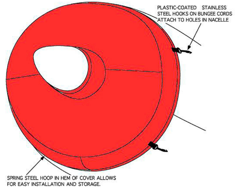
Intake Covers for Lockheed C-141
